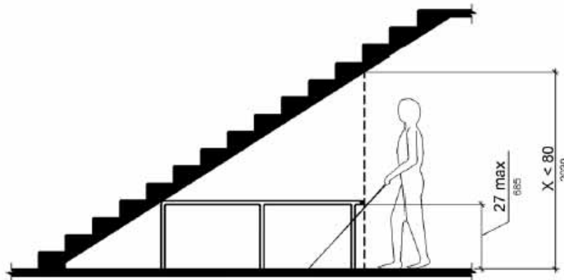
Figure 307.4 Vertical Clearance
