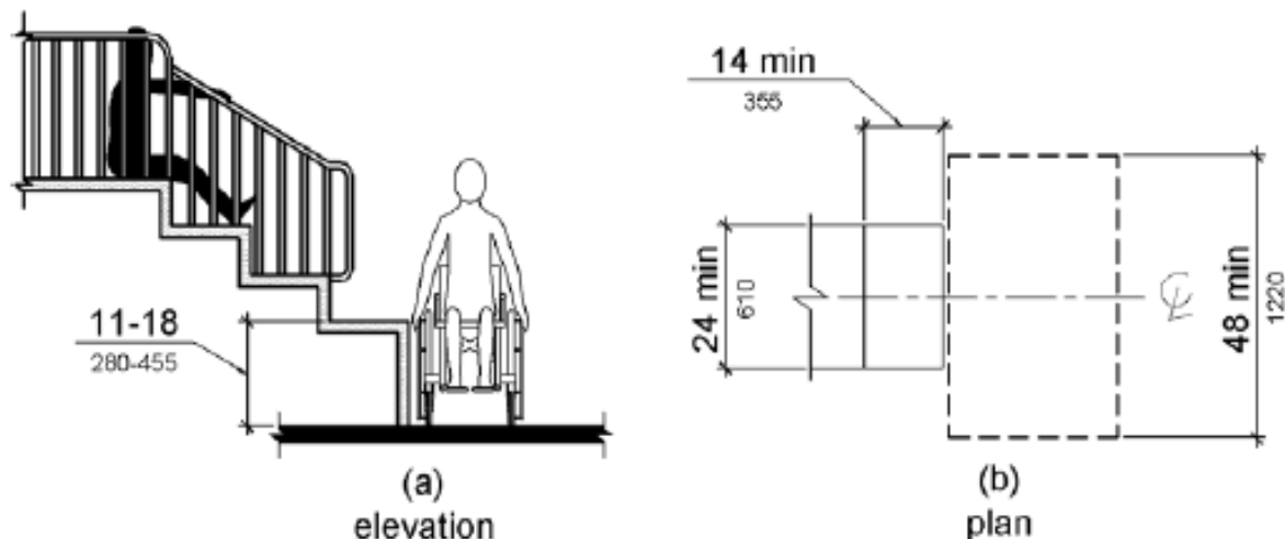
Figure 1008.3.1 Transfer Platforms
