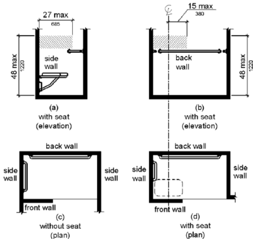
Figure 608.5.3 Alternate Roll-In Type Shower Compartment Control Location
