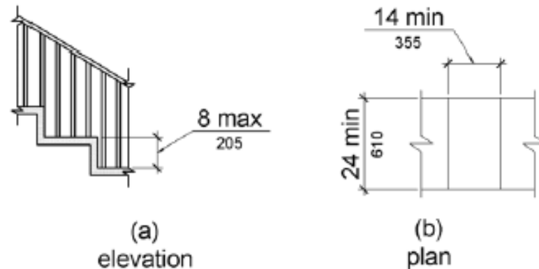
Figure 1008.3.2 Transfer Steps
