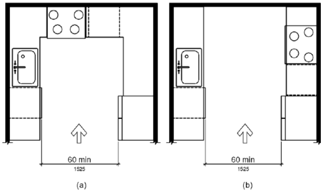
Figure 804.2.2 U-Shaped Kitchens
