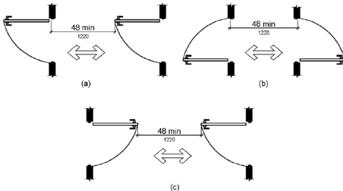
Figure 404.2.6 Doors in Series and Gates in Series
