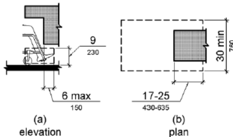
Figure 306.2 Toe Clearance
