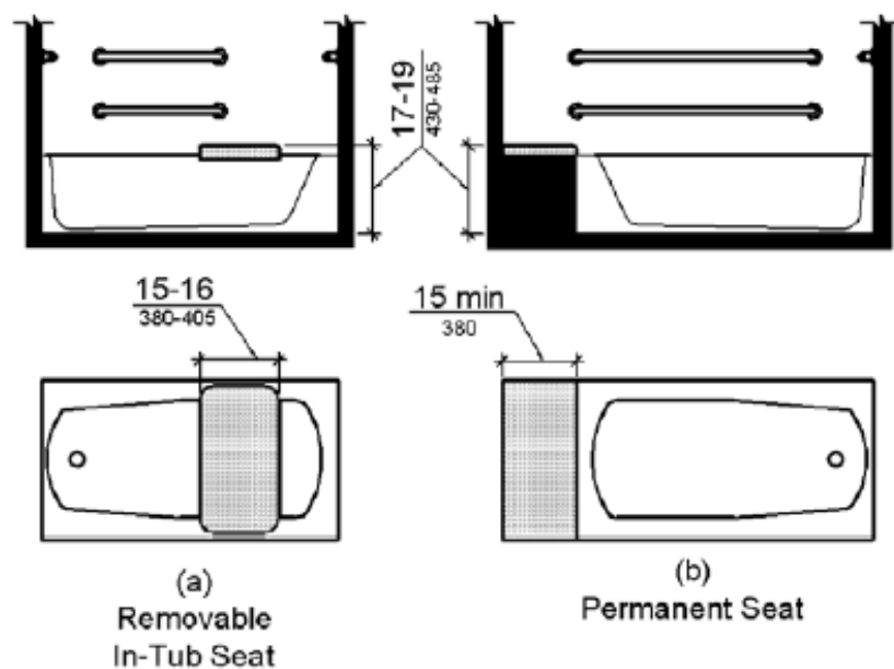
Figure 610.2 Bathtub Seats
