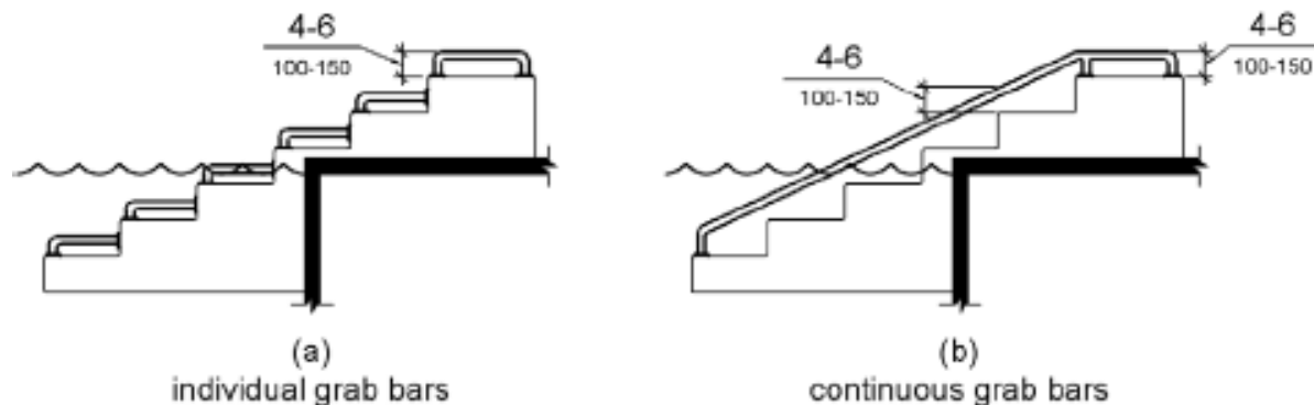
Figure 2009.5.7 Grab Bars
