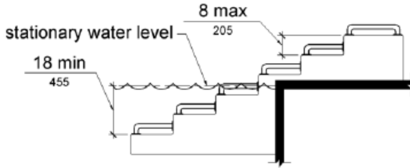
Figure 1009.5.4 Transfer Steps
