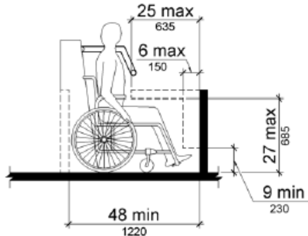
Figure 1002.4.4.3 Protrusions in Wheelchair Spaces in Amusement Rides
